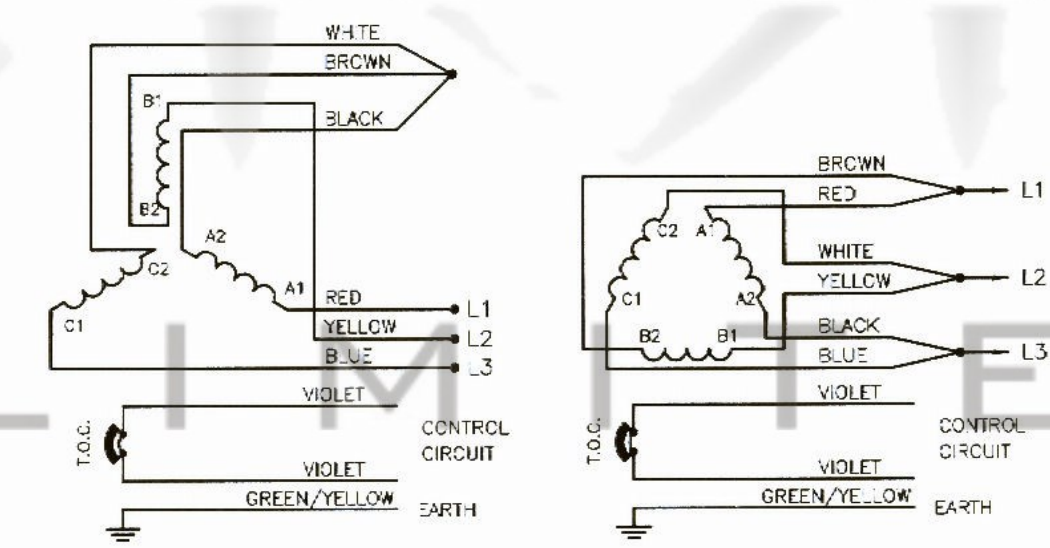
CONNECTION DIAGRAM
