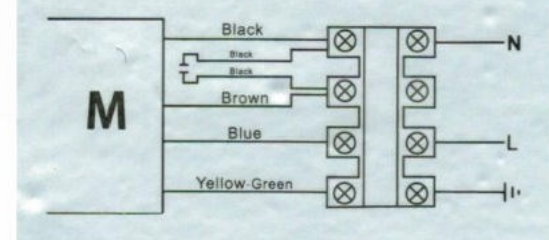
SINGLE-PHASE WIRING DIAGRAM
