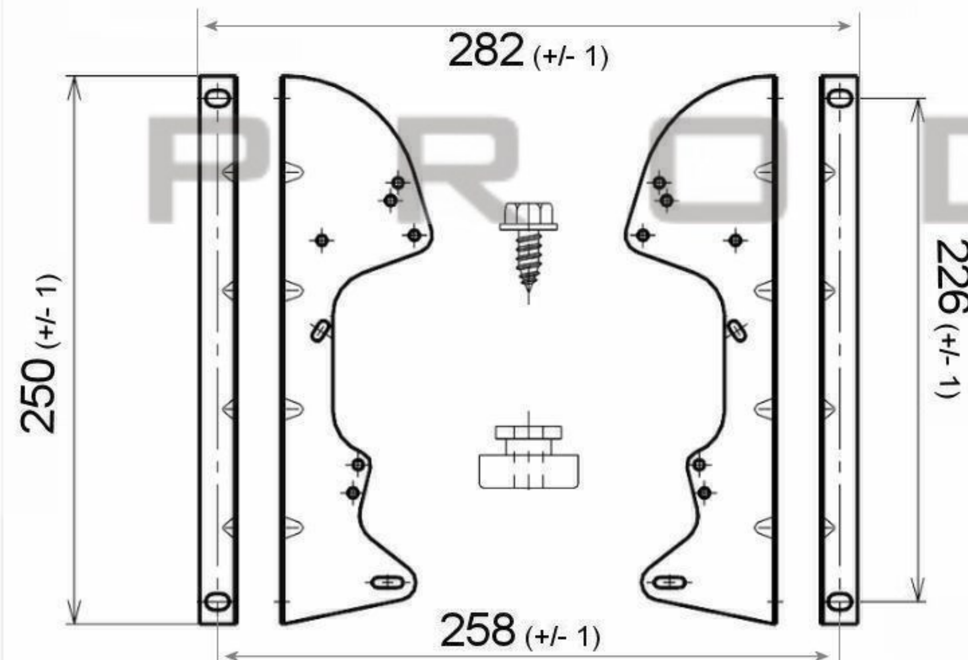
Accessories - DD7F (Mounting Feet)
