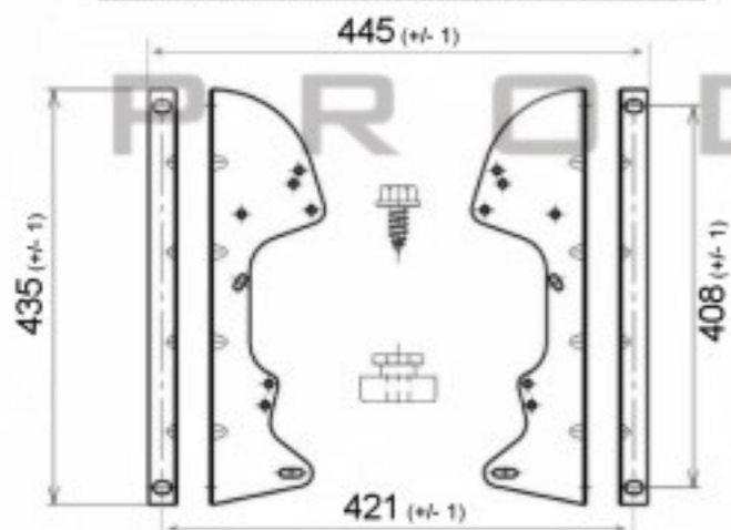
Accessories: DD12F (Mounting Feet)
