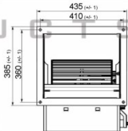
Accessories: DDF12/12 (Mounting Flange)
