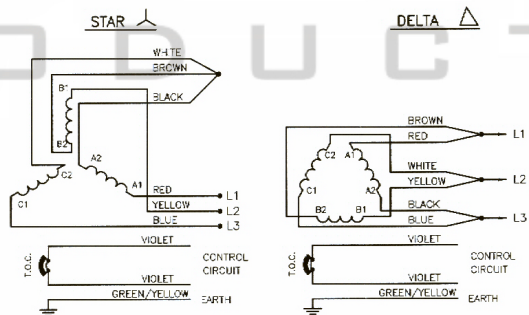
CONNECTION DIAGRAM
