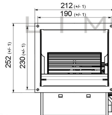
Accessories - DDF7/5 (Flange)
