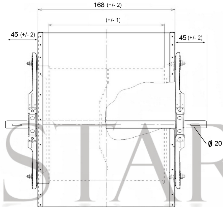
Accessories - DDF7/5 (Flange)
