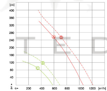
A: 2-Pole 50Hz, B: 2-Pole 60Hz C: 4-Pole 50 Hz, D: 4-Pole 60Hz
