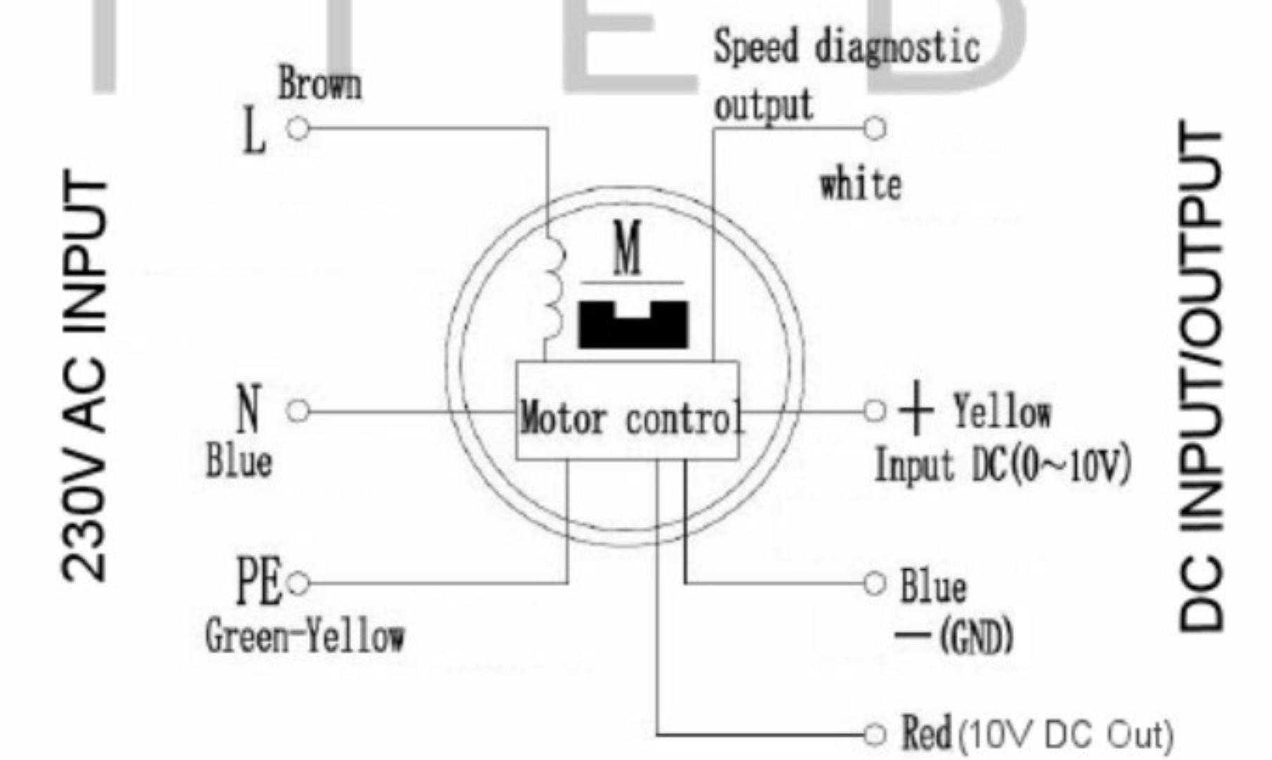
Motor Connection Diagram
