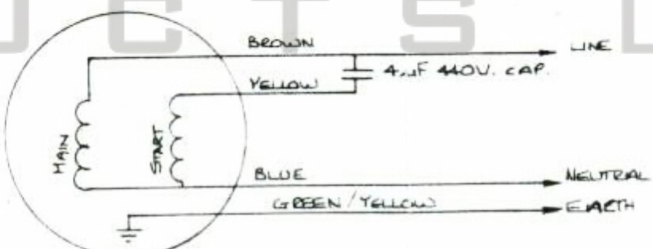
CONNECTION DIAGRAM
