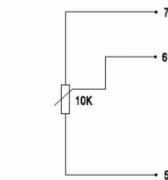
Air flow by using 0-10k variable resistance
