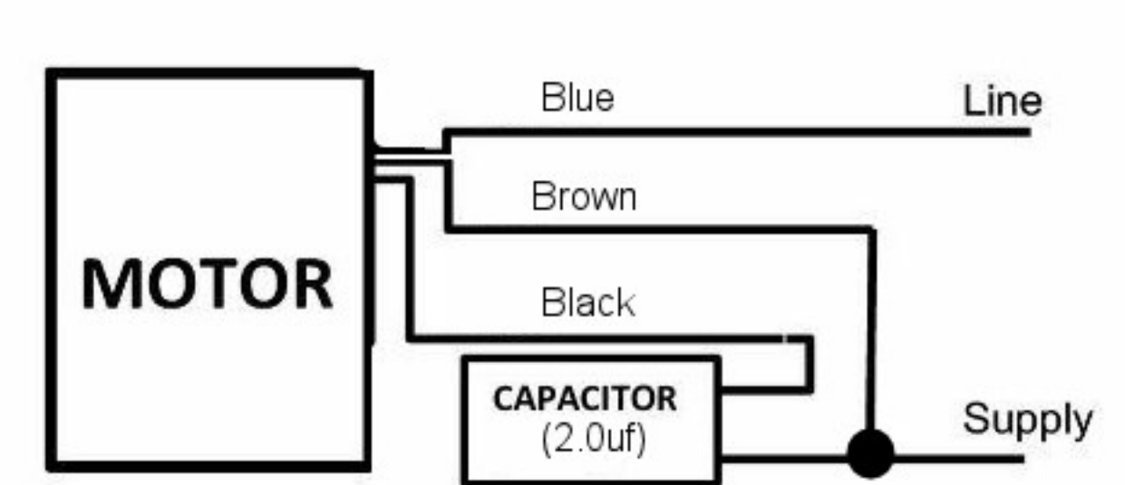
CLOCKWISE ROTATION
